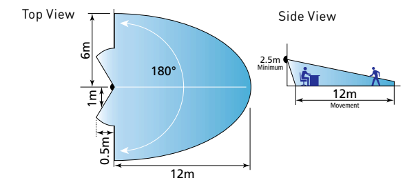
LED400PIR detection range and coverage.
