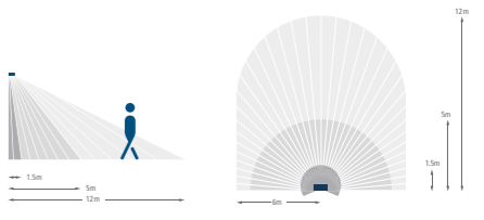
theLuxa S180 detection range and coverage.
