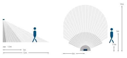
theLuxa S150 detection range and coverage.
